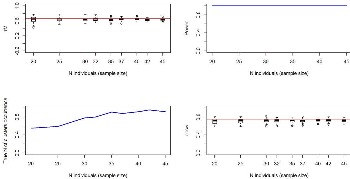
Figure 16620-3. Top left: simulated distribution (boxplots) and observed value (red line) of connectivity. Top right: Simulated power of the analysis. Bottom left: Proportion of times the analysis provides the
