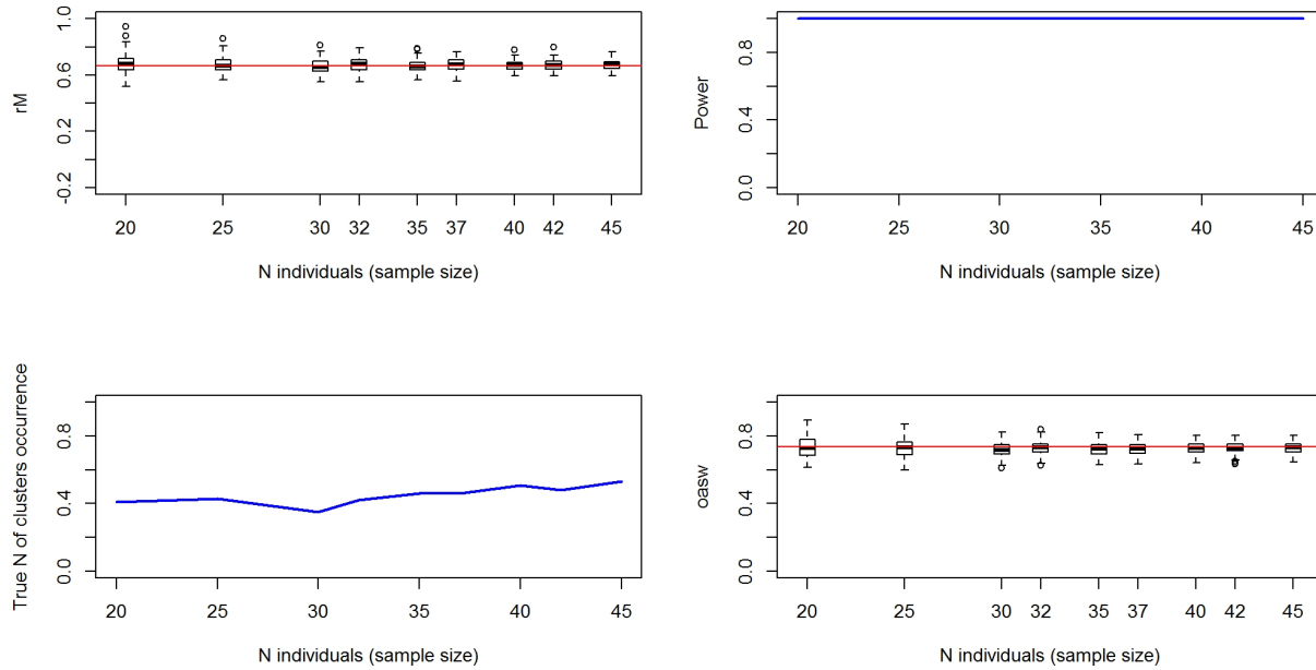
Figure 16620-2. Top left: simulated distribution (boxplots) and observed value (red line) of connectivity. Top right: Simulated power of the analysis (i.e. proportion of times the analyses on the subset of individuals was significant). Bottom left: Proportion of times the analysis provides the observed best number of cluster. Bottom right: simulated distribution (boxplots) and observed value (red line) of clustering intensity.
