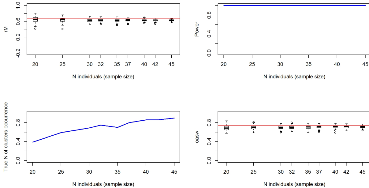
Figure 16620-4. Top left: simulated distribution (boxplots) and observed value (red line) of connectivity. Top right: Simulated power of the analysis. Bottom left: Proportion of times the analysis provides the observed best number of cluster. Bottom right: simulated distribution (boxplots) and observed value (red line) of clustering intensity.
