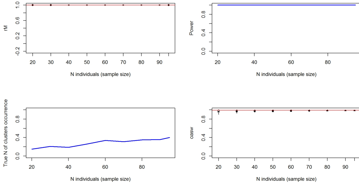
Figure 15920-2. Top left: simulated distribution (boxplots) and observed value (red line) of connectivity. Top right: Simulated power of the analysis (i.e. proportion of times the analyses on the subset of individuals was significant). Bottom left: Proportion of times the analysis provides the observed best number of cluster. Bottom right: simulated distribution (boxplots) and observed value (red line) of clustering intensity.
