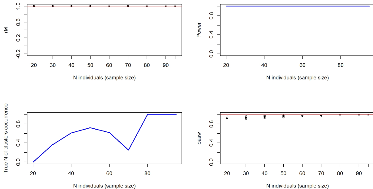
Figure 15920-3. Top left: simulated distribution (boxplots) and observed value (red line) of connectivity. Top right: Simulated power of the analysis. Bottom left: Proportion of times the analysis provides the
