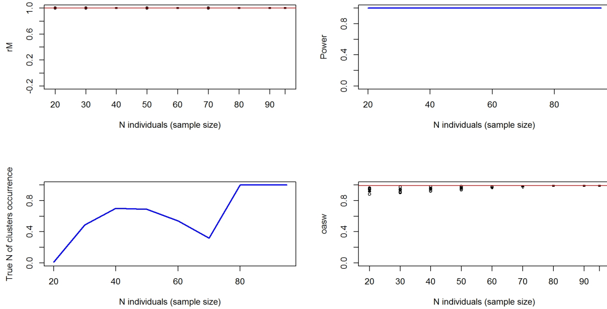
Figure 15920-4. Top left: simulated distribution (boxplots) and observed value (red line) of connectivity. Top right: Simulated power of the analysis. Bottom left: Proportion of times the analysis provides the observed best number of cluster. Bottom right: simulated distribution (boxplots) and observed value (red line) of clustering intensity.
