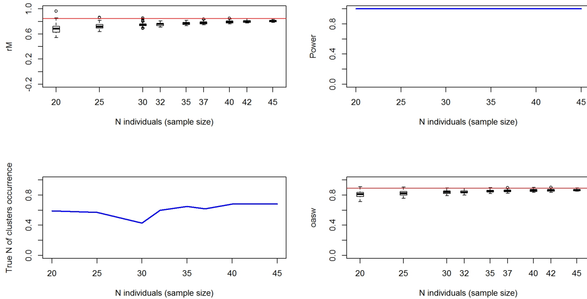
Figure 04770-4. Top left: simulated distribution (boxplots) and observed value (red line) of connectivity. Top right: Simulated power of the analysis. Bottom left: Proportion of times the analysis provides the observed best number of cluster. Bottom right: simulated distribution (boxplots) and observed value (red line) of clustering intensity.
