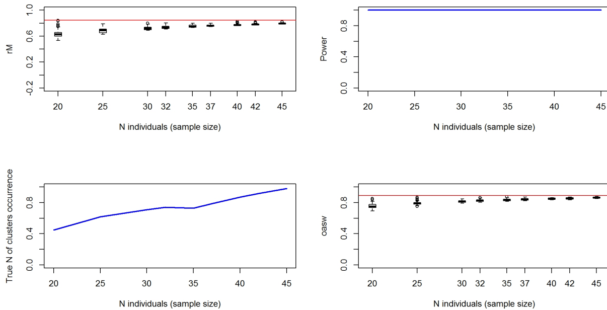
Figure 04770-3. Top left: simulated distribution (boxplots) and observed value (red line) of connectivity. Top right: Simulated power of the analysis. Bottom left: Proportion of times the analysis provides the
