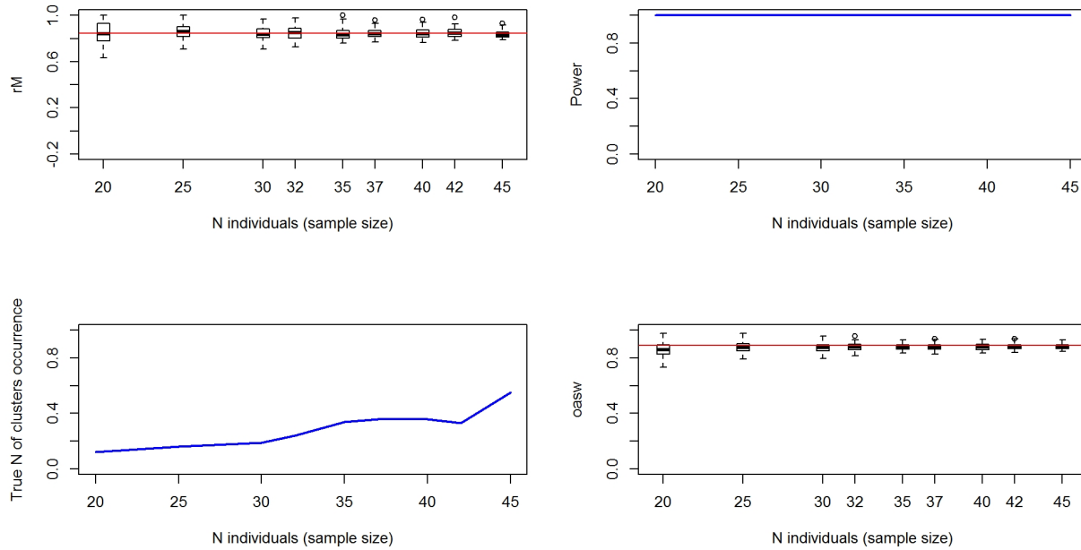
Figure 04770-2. Top left: simulated distribution (boxplots) and observed value (red line) of connectivity. Top right: Simulated power of the analysis (i.e. proportion of times the analyses on the subset of individuals was significant). Bottom left: Proportion of times the analysis provides the observed best number of cluster. Bottom right: simulated distribution (boxplots) and observed value (red line) of clustering intensity.
