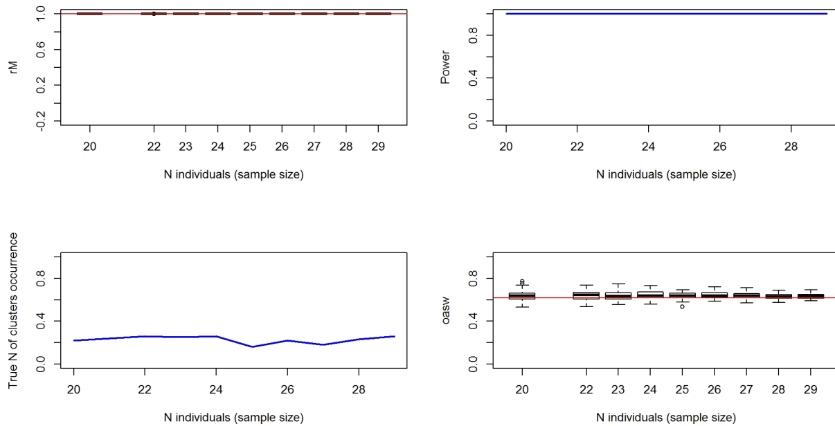
Figure 03350-3. Top left: simulated distribution (boxplots) and observed value (red line) of connectivity. Top right: Simulated power of the analysis. Bottom left: Proportion of times the analysis provides the
