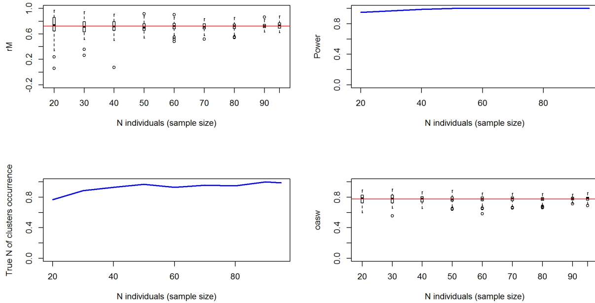
Figure 01570-2. Top left: simulated distribution (boxplots) and observed value (red line) of connectivity. Top right: Simulated power of the analysis (i.e. proportion of times the analyses on the subset of individuals was significant). Bottom left: Proportion of times the analysis provides the observed best number of cluster. Bottom right: simulated distribution (boxplots) and observed value (red line) of clustering intensity.
