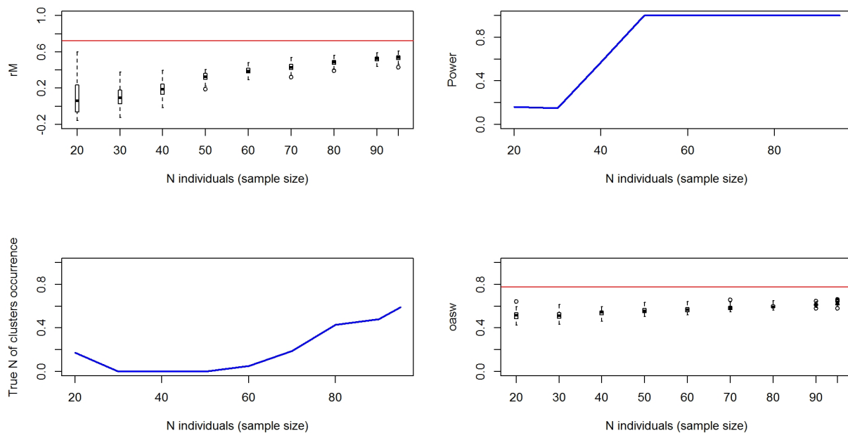
Figure 01570-3. Top left: simulated distribution (boxplots) and observed value (red line) of connectivity. Top right: Simulated power of the analysis. Bottom left: Proportion of times the analysis provides the
