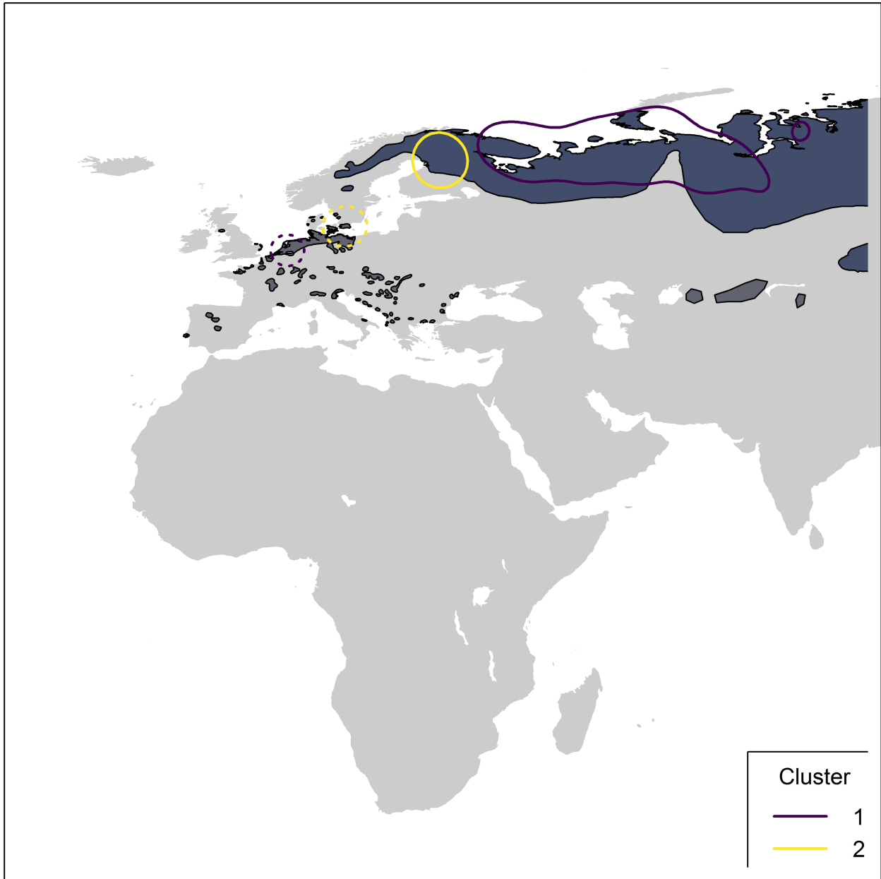
Figure 01570-1. Map showing 95% kernel contours of of first-level clusters identified by the migratory connectivity analysis, if any, or 95% kernel contours of all encounters, in case of no clustering structure. Solid lines indicate the clusters in the breeding range, dotted lines those in the non-breeding range. Different contour colours correspond to different clusters, as reported in legend. The species distribution range is also shown (breeding range: blue; non-breeding range: dark grey; resident range: beige; from BirdLife International, 2019).
