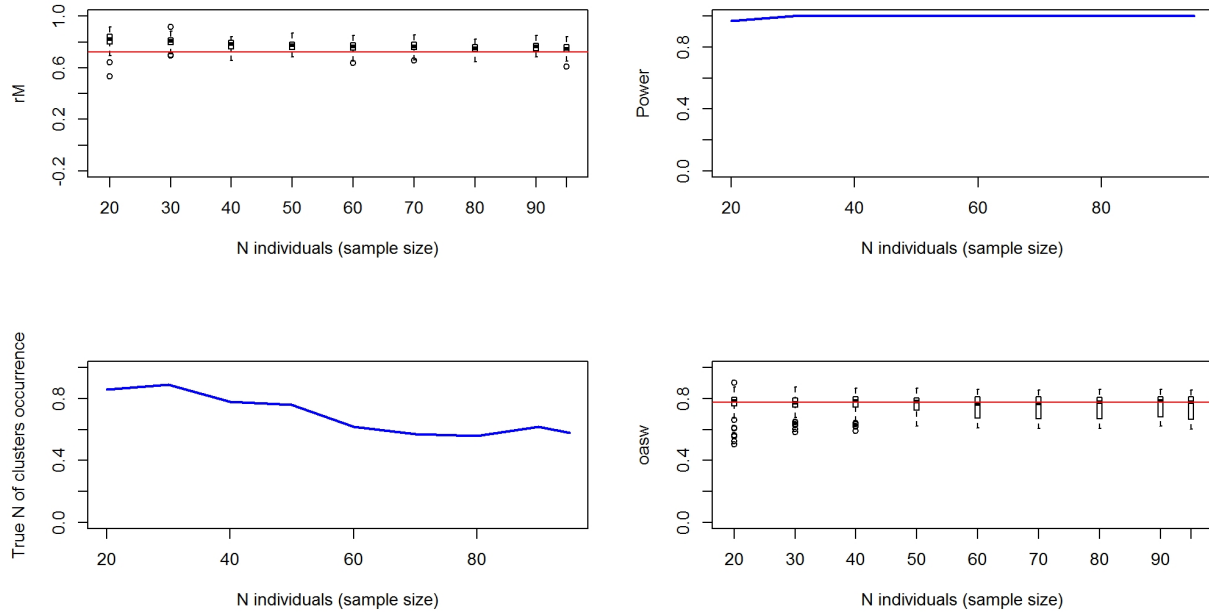
Figure 01570-4. Top left: simulated distribution (boxplots) and observed value (red line) of connectivity. Top right: Simulated power of the analysis. Bottom left: Proportion of times the analysis provides the observed best number of cluster. Bottom right: simulated distribution (boxplots) and observed value (red line) of clustering intensity.
