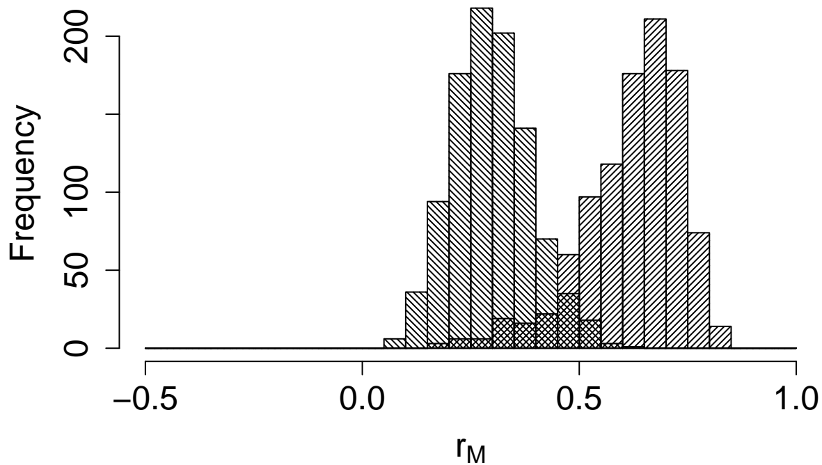
Figure 01570-5. Comparison between the bootstrapped distributions of connectivity value for alive recaptures (filling lines with angle=45°) and dead recoveries (filling lines with angle=375°).
